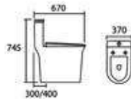
Siphonic one-piece toilet Bowl & Tank Size : 670 x 370 x 745 mm S-trap, 300 mm Roughing-in
