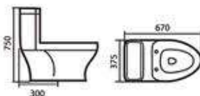
Siphonic one-piece toilet Size : 670 x 375 x 750 mm S-trap, 300 mm Roughing-in
