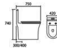
Siphonic one-piece toilet Bowl & Tank Size : 750 x 420 x 740 mm S-trap, 300 mm Roughing-in
